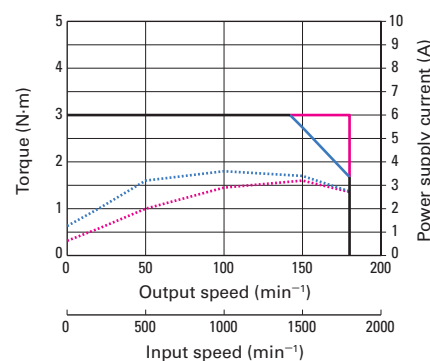
③ Motor model number PBM603DGER60
