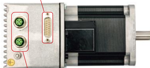
M12 EtherCAT IN / OUT connectors
